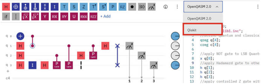
Fig. 30.1 QPE circuit to find the phase of the Z-gate's eigenvalue using a 3-qubit c-register
