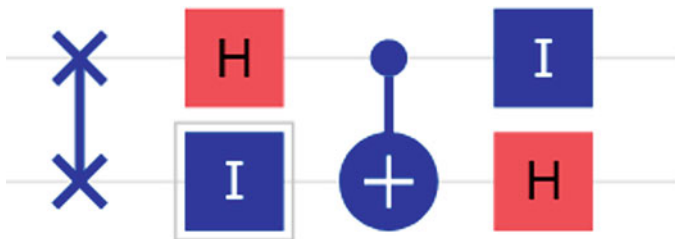
Fig. B.3 Circuit for question QB.29b
