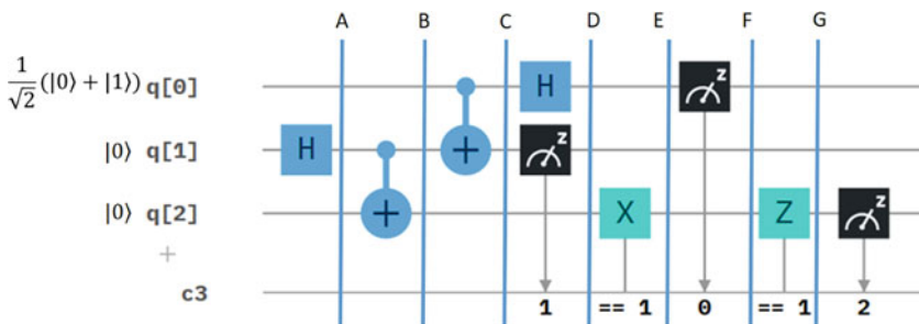
Fig. B.6 Circuit for question QB.35
