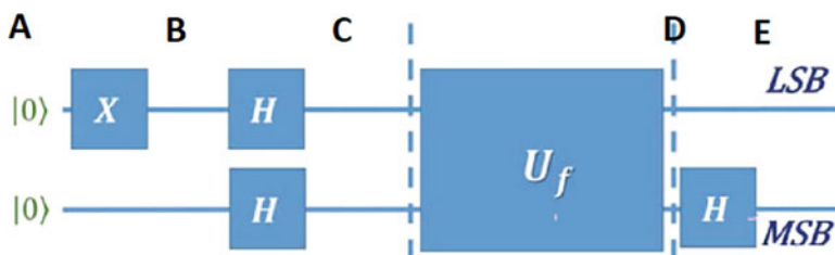
Fig. B.10 Circuit for question QB.40
