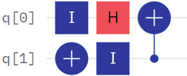
Fig. B.5 Circuit for question QB.32a
