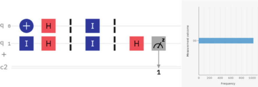
Fig. C.3 Circuit and result for question QC.20a
