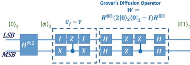
Fig. 24.1 Circuit to implement the Grover's algorithm for the given example
