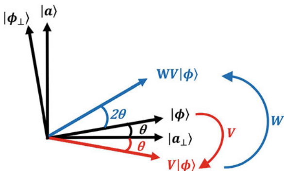
Fig. 23.2 Illustration of the Grover's algorithm. The first two steps are shown.
