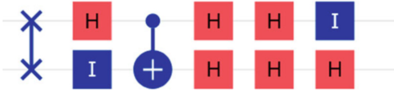
Fig. B.4 Circuit for question QB.29d
