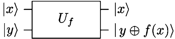
Fig. B.9 Circuit for question QB.38
