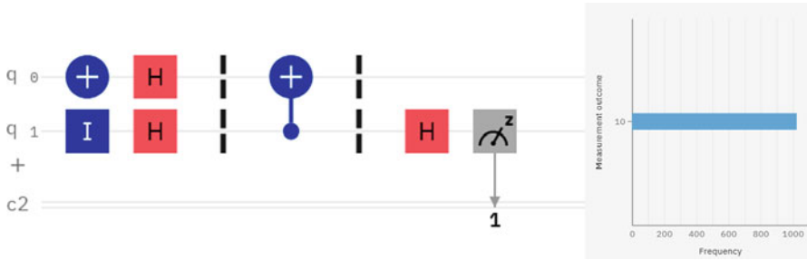
Fig. C.5 Circuit and result for question QC.20c
