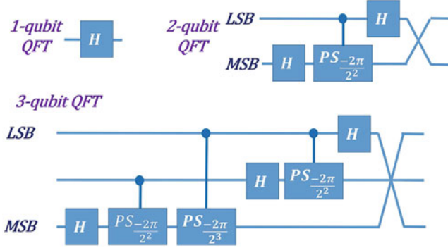
Fig. 26.4 Quantum circuits of 1-, 2-, and 3-qubit QFT
