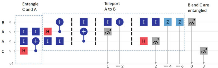
Fig. C.1 Circuit for question C.19
